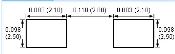
Solder Pads Unit: inch (mm)
