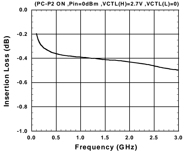
PC-P2 Insertion Loss vs. Frequency
