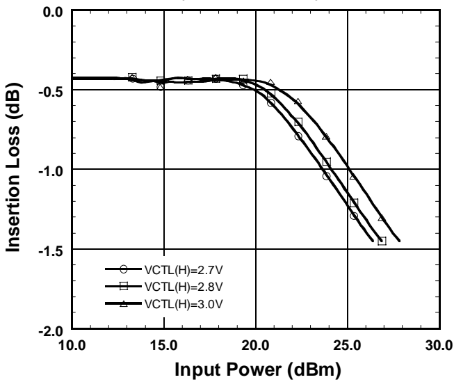
Insertion Loss vs. Input Power
