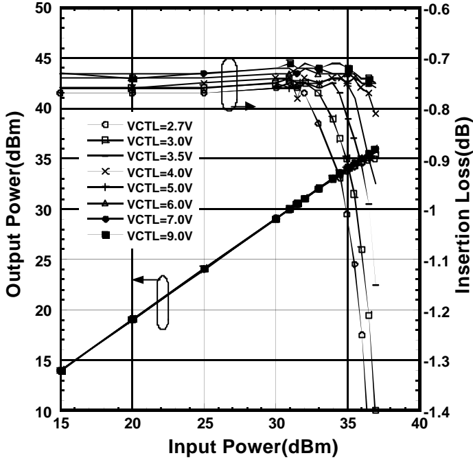
Output Power, Insertion Loss vs. Input power (PC-P1, f=2GHz)
