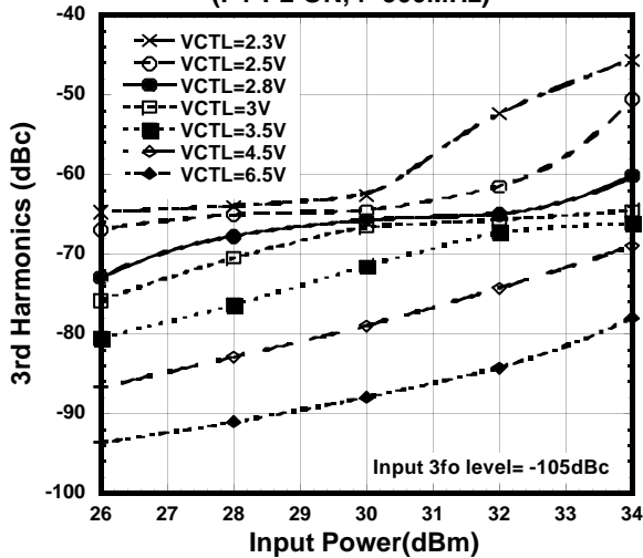
3rd Harmonics vs.Input Power (P1-P2 ON, f=900MHz)
