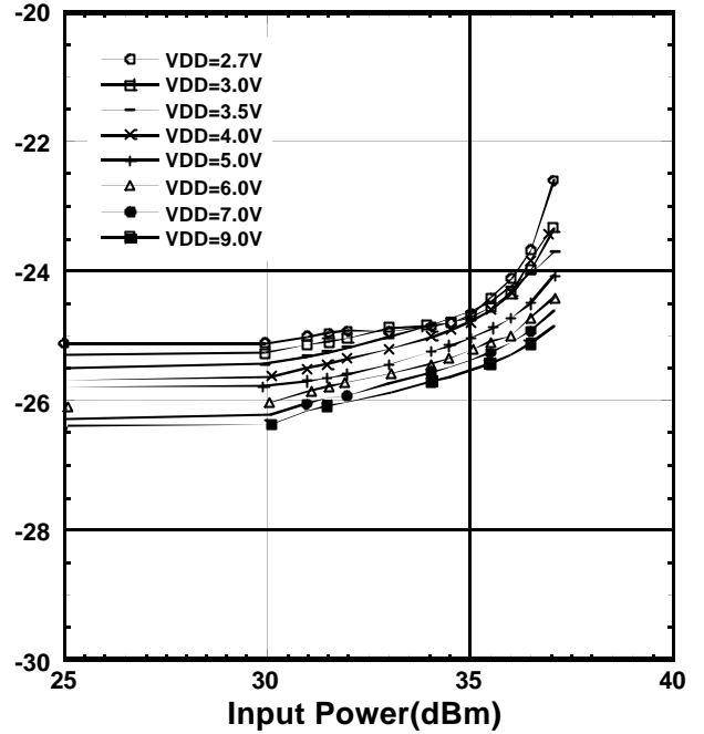
PC-P1 Isolation vs. Input Power (PC-P1, f=2\text{GHz} )
