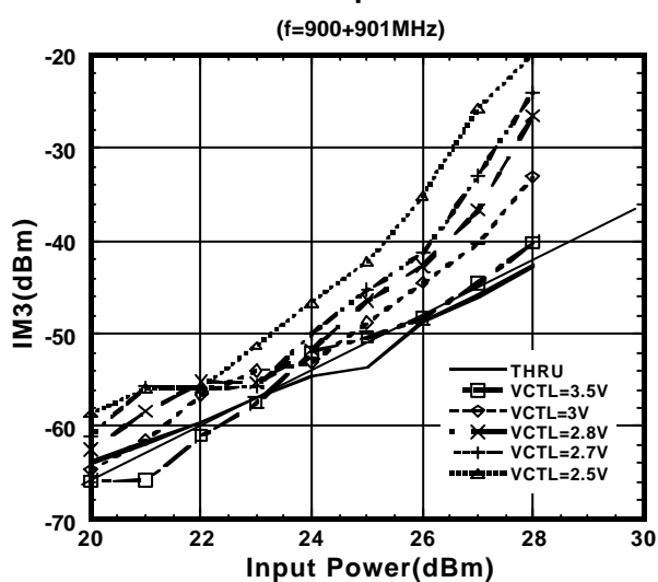
IM3 vs. Input Power
