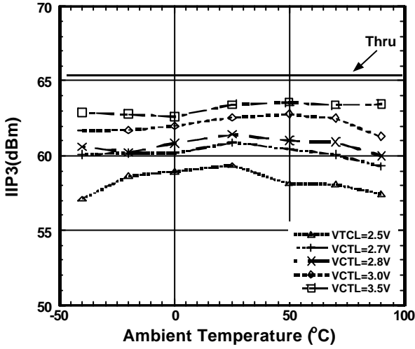
IIP3 vs. Ambient Temperature (PC-P1, f=900+901MHz, Input Power=25dBm)
