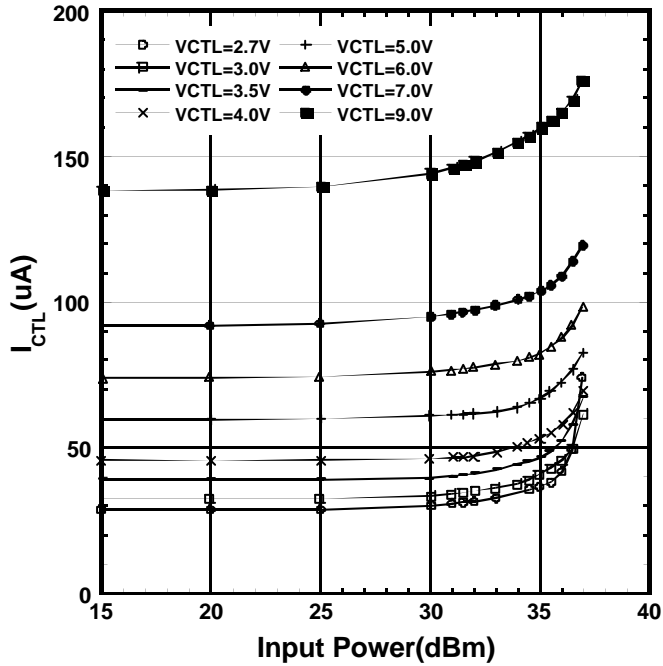
I_{CTL} vs. Input Power (PC-P1, f=2\text{GHz} )
