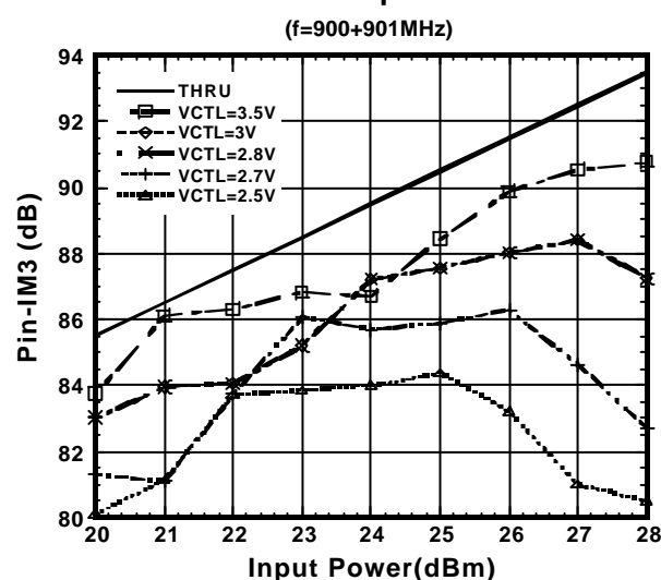
Pin-IM3 vs. Input Power
