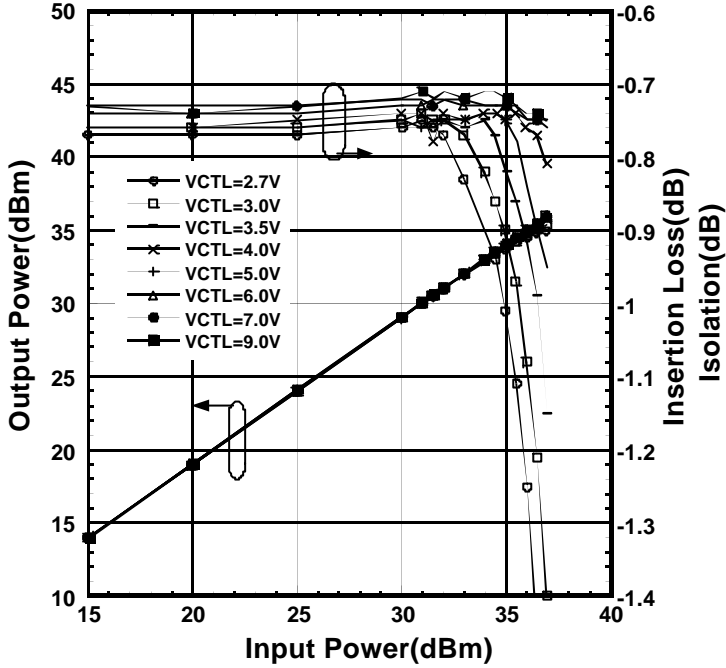
Output Power, Insertion Loss vs. Input power (PC-P1, f=2\text{GHz} )
