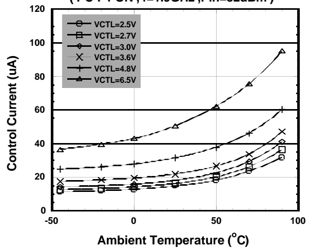
Control Current vs. Ambient Temperature ( PC-P1 ON , f=1.9GHz , Pin=32dBm )
