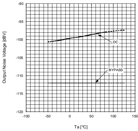
Output vs. Temperature
