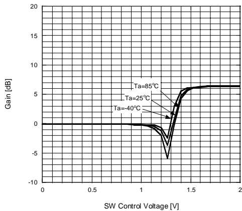
Gain vs. SW Control Voltage
