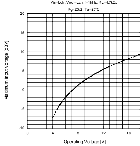
Maximum Input Voltage vs. Operating Voltage (DC)
