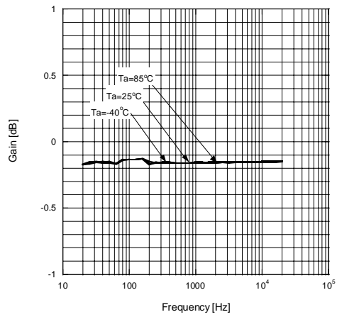
Frequency Response (BYPASS)
