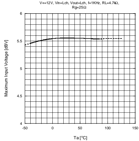
Maximum Input Voltage vs. Temperature (DC)
