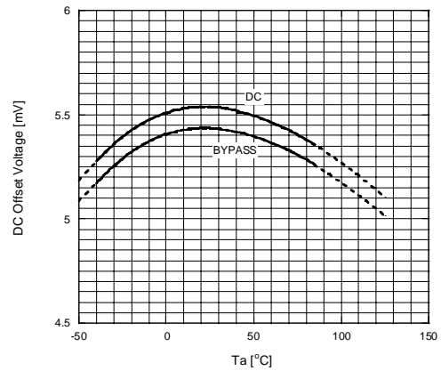
DC Offset Voltage vs. Temperature
