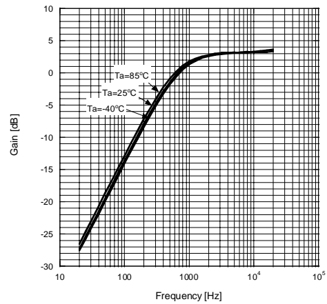
Frequency Response (DC)
