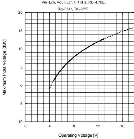
Maximum Input Voltage vs. Operating Voltage (BYPASS)
