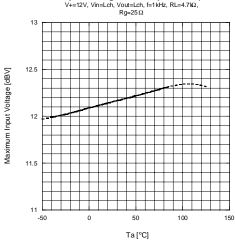
Maximum Input Voltage vs. Temperature (BYPASS)
