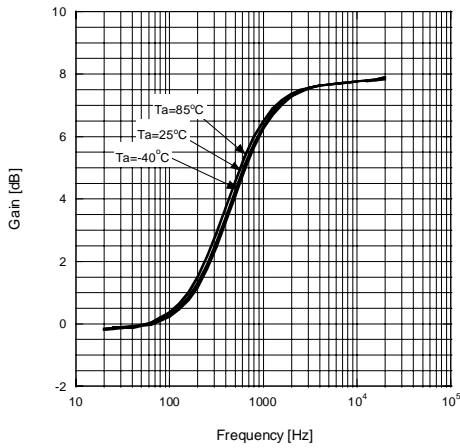
Frequency Response (DC)
