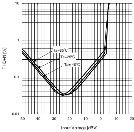
Total Harmonic Distortion vs. Input Voltage (DC)
