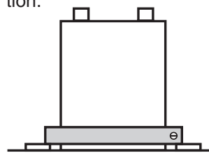
Clip mounted: R_{th} = 3.6^\circ\text{C}/\text{W}
