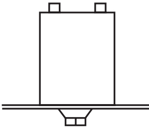
Stud mounted: R_{th} = 2.1^{\circ}\text{C/W}
