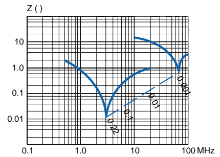
Resonance frequencies CMK 5
